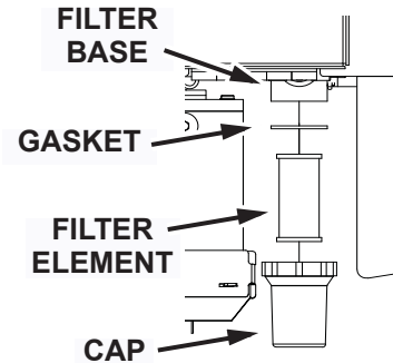
Fig. 2: Water Solution Filter with Exploded view
