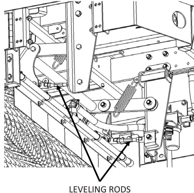
Fig. 4: Leveling Rod location
