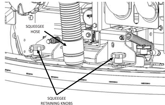
Fig. 1: Turning/Replacing the Rear Squeegee Blades
