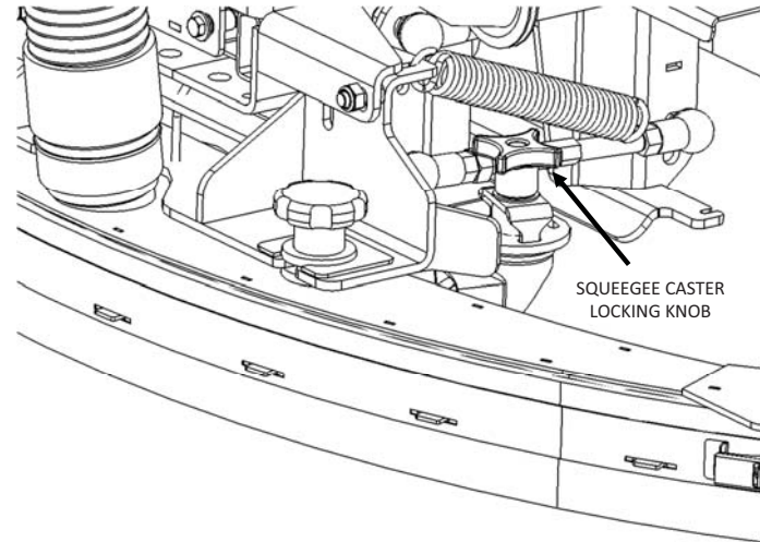
Fig. 1: Adjusting the Rear Squeegee Blade Flair
