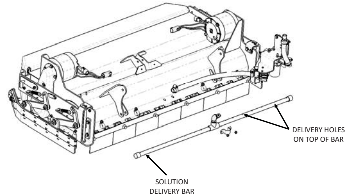
Fig. 1: Solution Delivery Bar shown with holes
