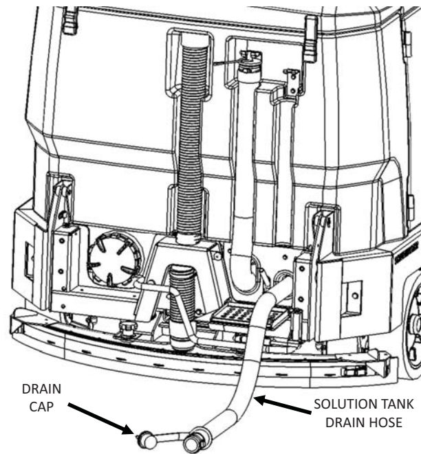
Fig. 1: Draining the Solution Tank
