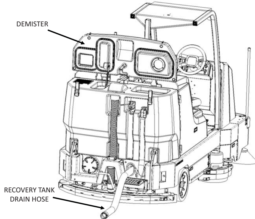
Fig. 1: Draining the Recovery Tank
